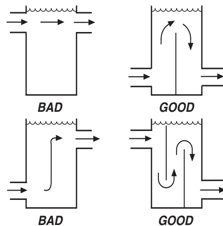
Fig. 35 — Tank Baffling
