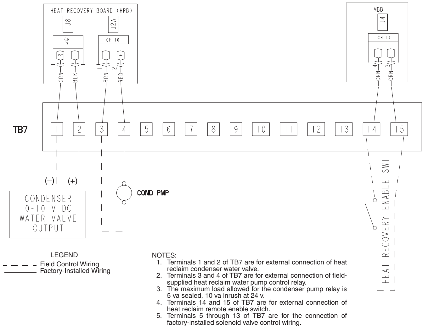
Fig. 59 — Optional Heat Reclaim Control Typical Field Wiring
