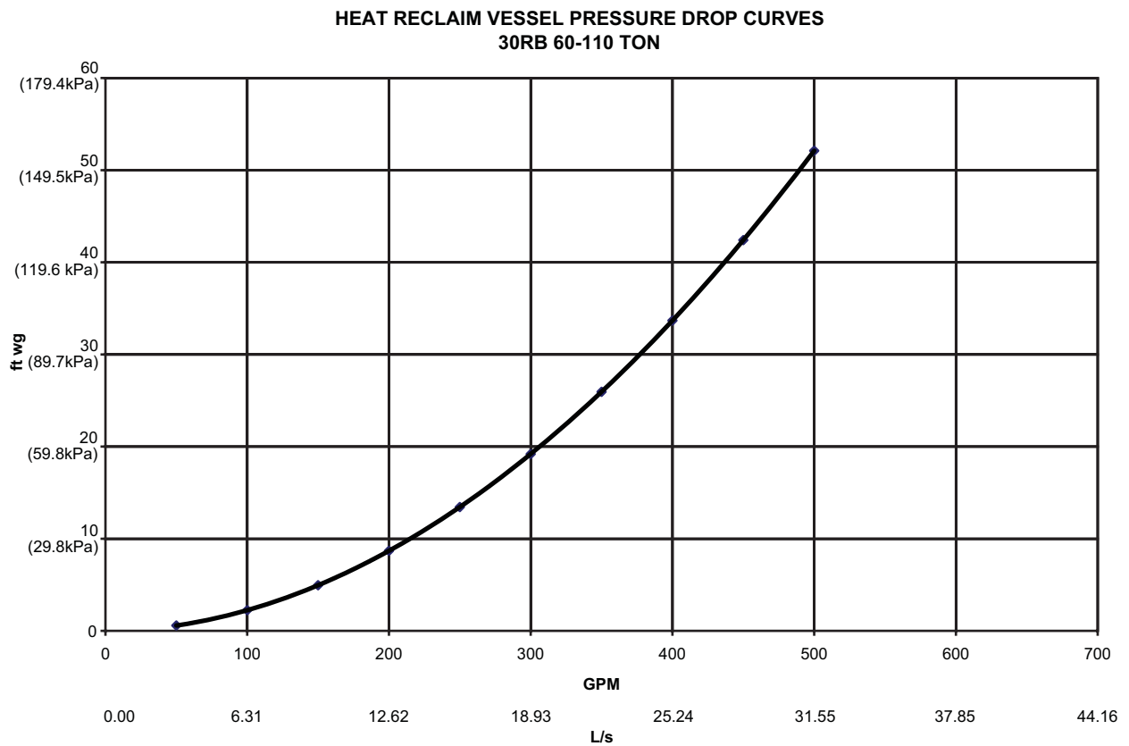
Fig. 55 — 30RB060-110 Optional Heat Reclaim Pressure Drop Curves
