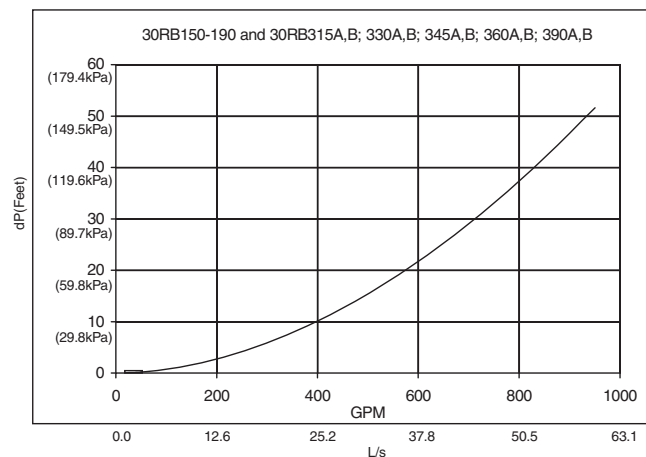
Fig. 53 — 30RB150-190 and 30RB315A,B; 330A,B; 345A,B; 360A,B; 390A,B Cooler Pressure Drop Curve
