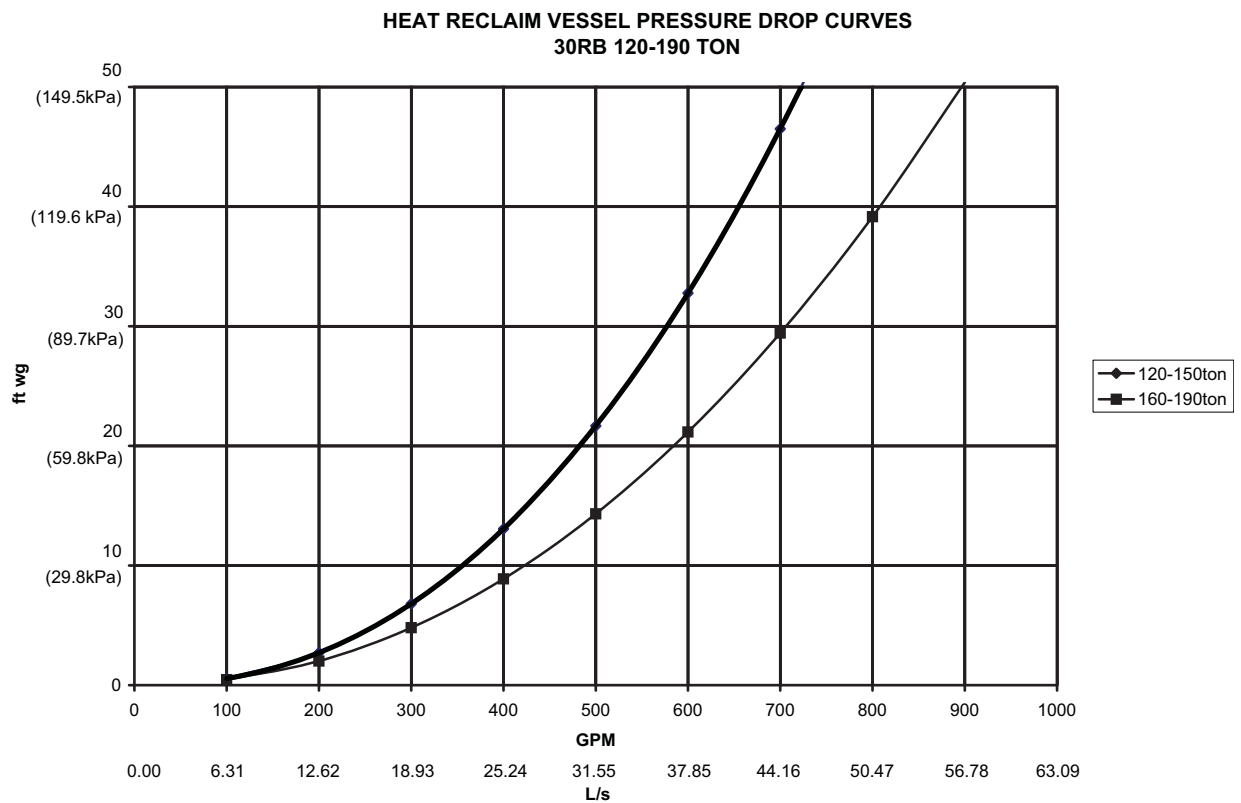
Fig. 56 — 30RB120-190 Optional Heat Reclaim Pressure Drop Curves
