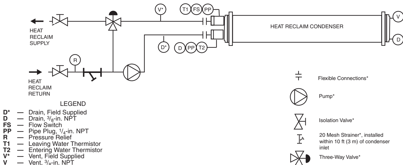
Fig. 31 — Typical Piping Diagram on 30RB Units without Hydronic Package
