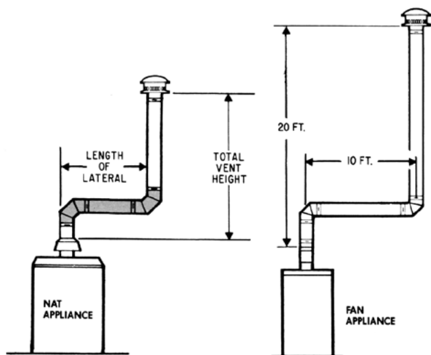
FIG 1 - INDIVIDUAL VENT-LATERAL AND HEIGHT
