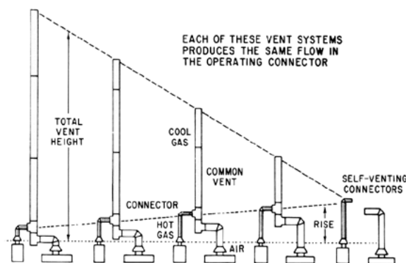
FIG. 9 - BENEFIT OF GREATER CONNECTOR RISE
