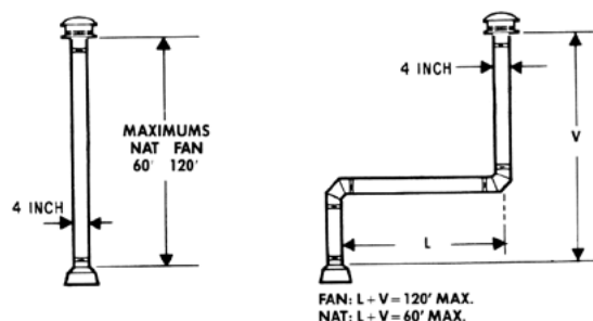
FIG. 6 - INDIVIDUAL VENT LENGTH LIMIT EXAMPLE
