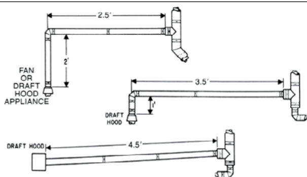
FIG. 7 - CONNECTOR LENGTH MEASUREMENT
