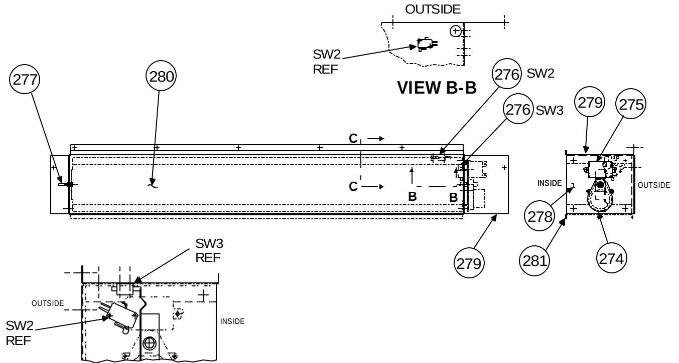
VIEW C-C
