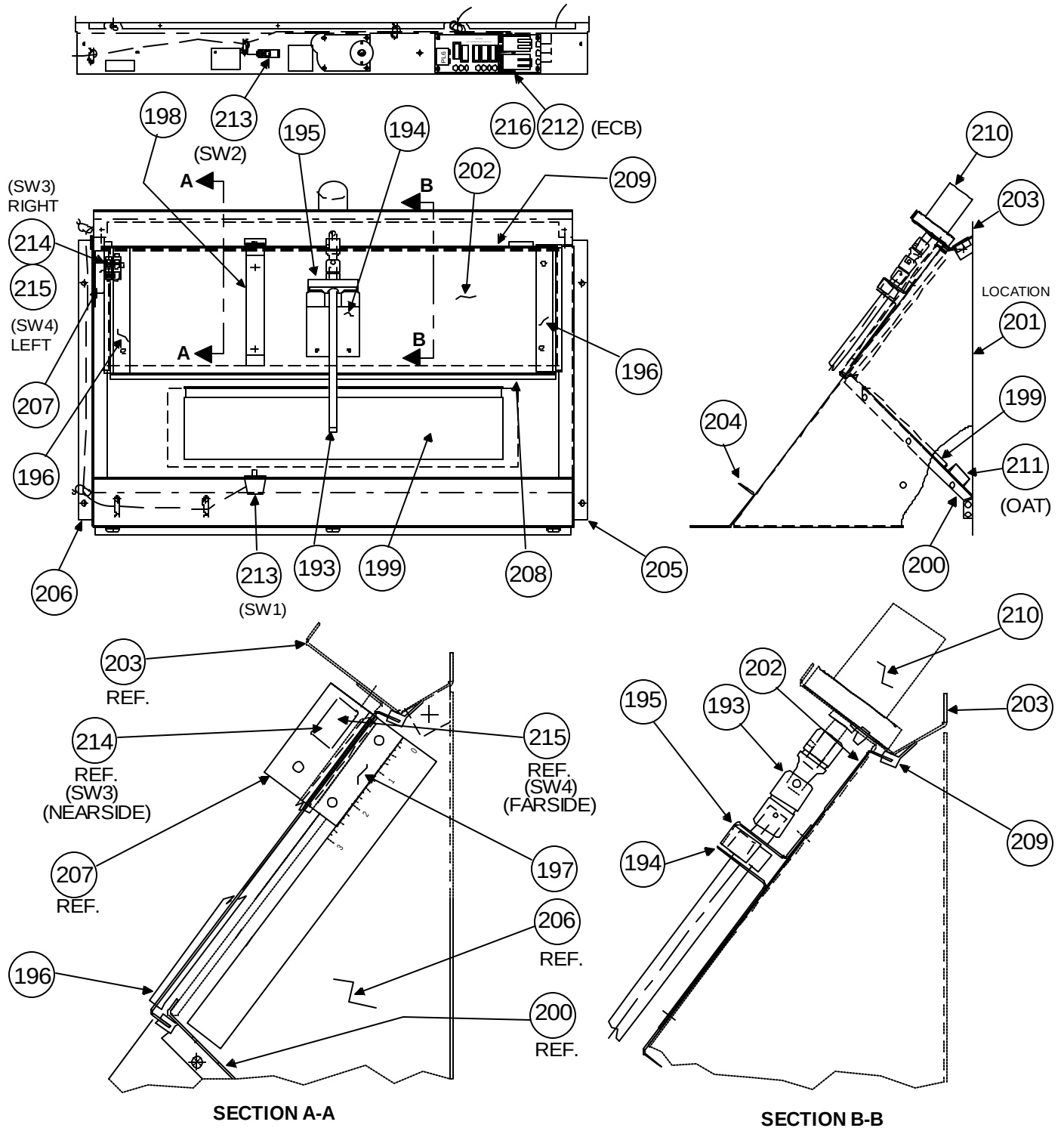
DURABLADE ECONOMIZER, ITEM 134 OR 265
