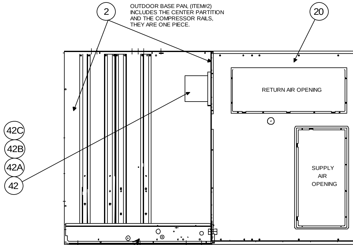
CONTROL BOX REF. OVERALL VIEW
