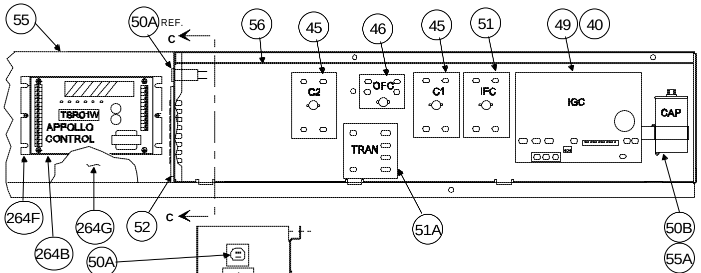
ELECRICAL BOX, COMPONENT ARRANGMENT
