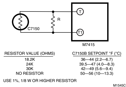
Fig. 19. Decreasing C7150B setpoint.
