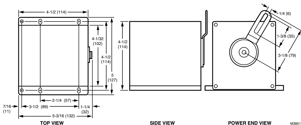
Fig. 4. Approximate dimensions of M7415A and M8405A in in. (mm).
