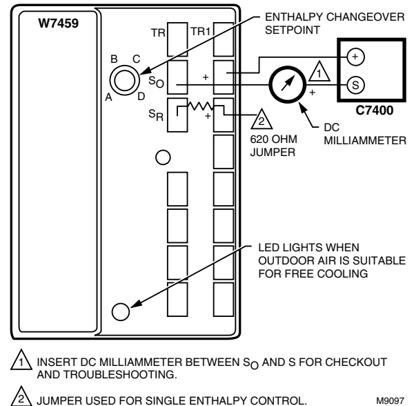
Fig. 21. Meter location for checkout and troubleshooting.
