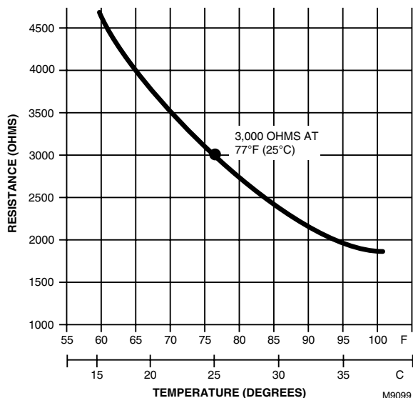
Fig. 14. C7046C and C7150B Air Temperature Sensors resistance versus temperature.
