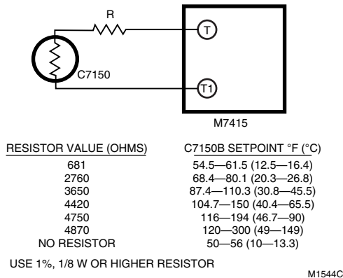
Fig. 18. Increasing C7150B setpoint.
