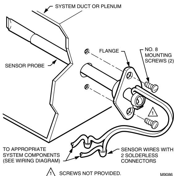
Fig. 7. Mounting C7046C Air Temperature Sensor on duct or plenum.
