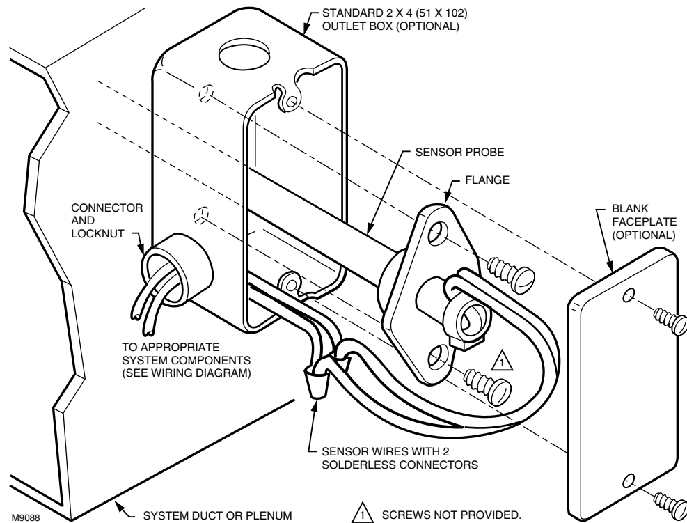
Fig. 8. Mounting C7046C Discharge Air Temperature Sensor in junction box.
