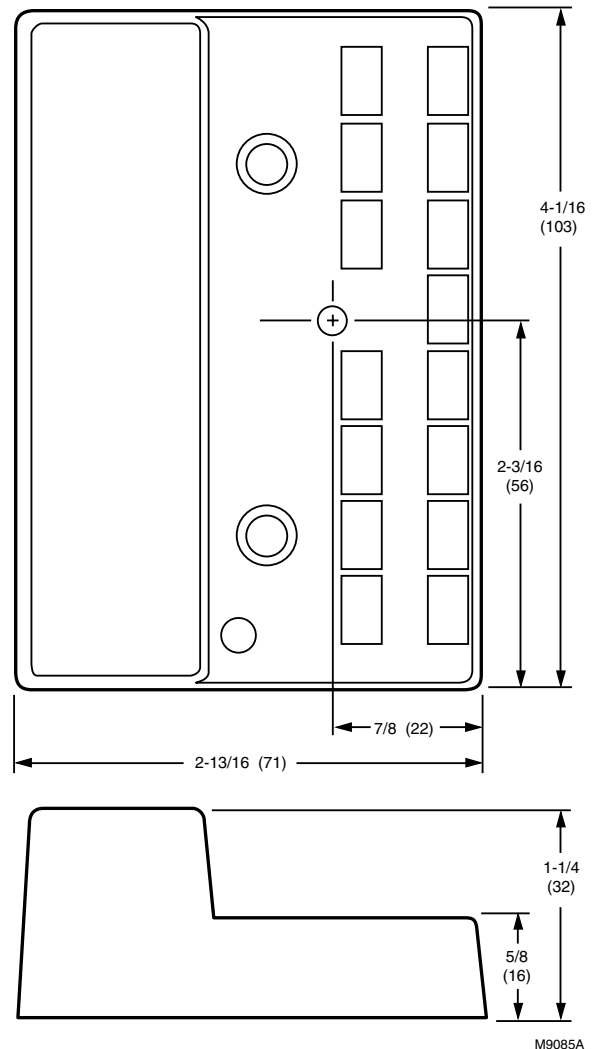
Fig. 6. Approximate dimensions of W7459 Solid State Economizer Logic Module in in. (mm).
