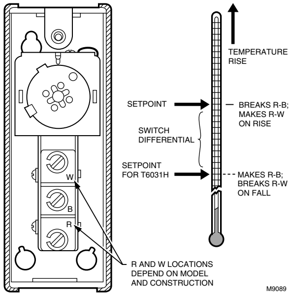
Fig. 11. T6031H switch terminal arrangement and switching.
