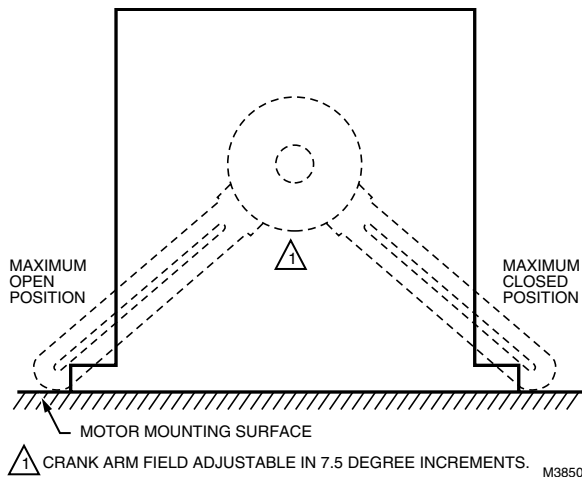
Fig. 9. Limits of crank arm rotation.
