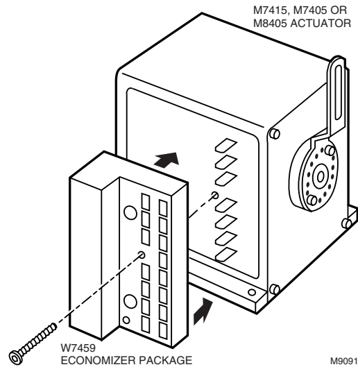
Fig. 12. Mounting W7459 on M7415 or M8405 Damper Actuator.
