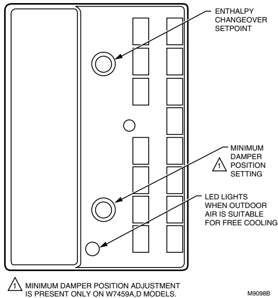
Fig. 20. Location of enthalpy setpoint potentiometer, minimum position potentiometer and LED.
