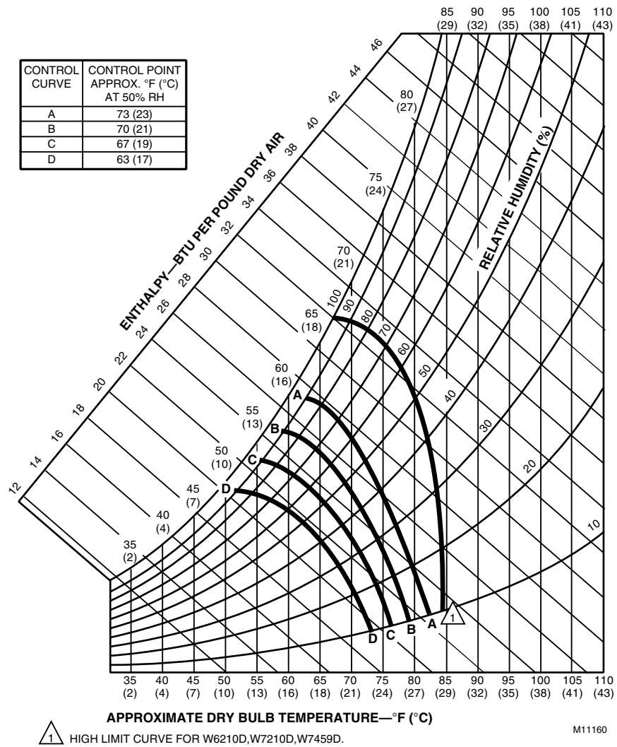
Fig. 15. Partial psychrometric chart with single C7400A Solid State Enthalpy Sensor and W7459 Solid State Economizer Logic Module performance curves.
