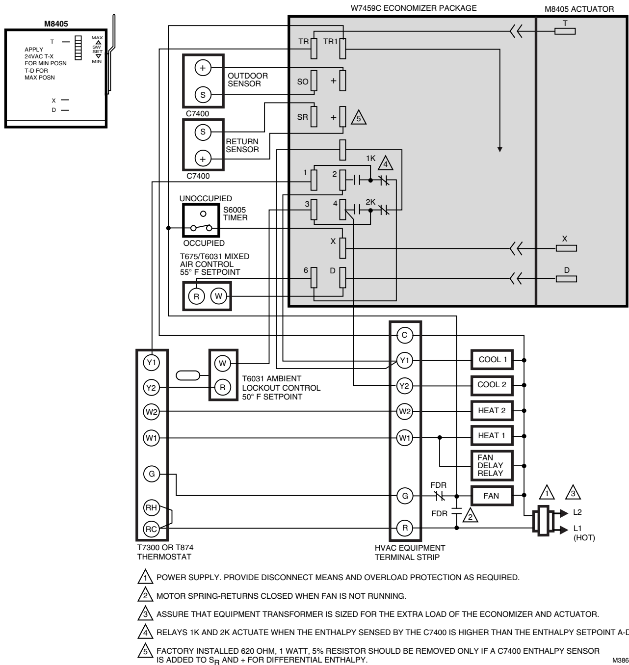
Fig. 10. M8405A Damper Actuator used in two-stage cooling system with differential enthalpy changeover and W7459C Economizer.
