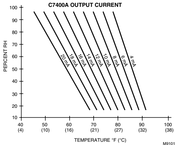
Fig. 16. C7400A Sensor output current vs. relative humidity.
