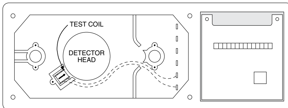
Figure 3. Test Coil Installation:
