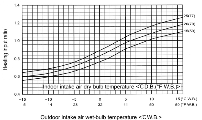
Fig. 2-2 Heating input
