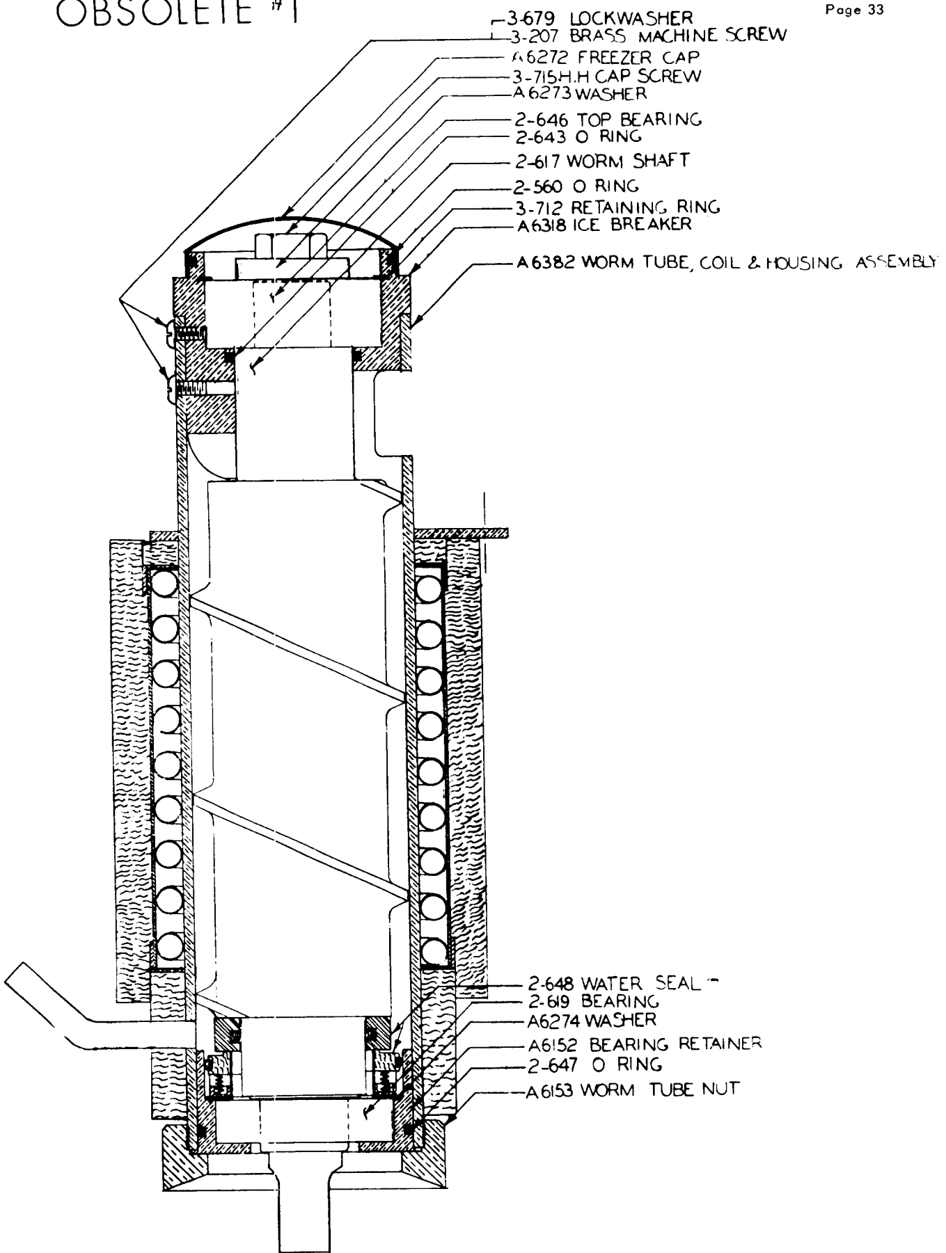
FREEZER ASSEMBLY SF- 2 F
