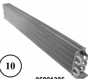
06001386 Evaporator Coil for Non Endwall Models BB48, BB60, BB72, BB84, ND48, ND40, ND52, ND60 ND72, KC48, KC72, KC84 (27-1/2" L, 4" H, 1-7/8" W)
